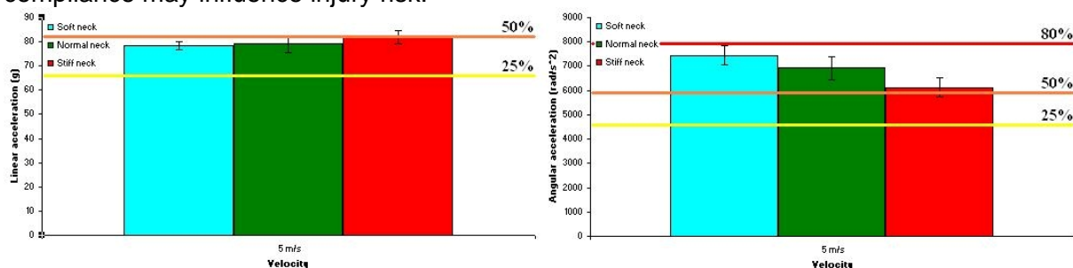
Figure 2: Peak linear acceleration and peak angular acceleration measured during a direct impact to the front of a Hybrid III head attached to necks with three different compliances at 5 m/s. The lines represent a 50% and 80% probability of sustaining an mTBI.
