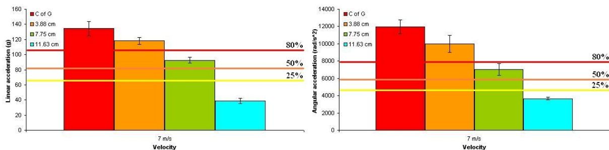
Figure 1: Peak linear acceleration and peak angular acceleration measured during front impacts through the centre of gravity plus three displacements at 7 m/s. The lines represent a 25%, 50% and 80% probability of sustaining an mTBI.
